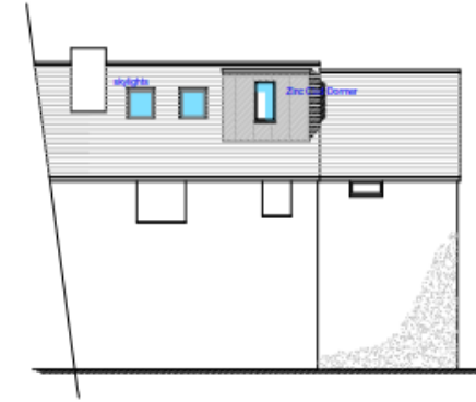
Proposed Rear Elevation 1:100
