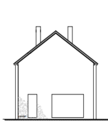
Left Elevation 1:100
