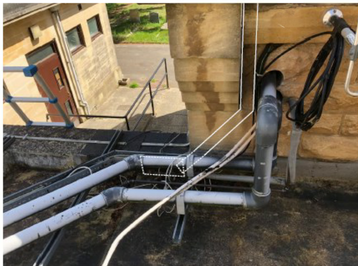
Figure 9. New downpipe to be installed and chute dressed in lead in parapet.
